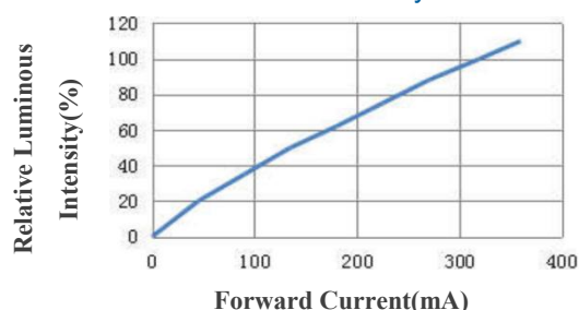
Relative Luminous Intensity -IF Curve
