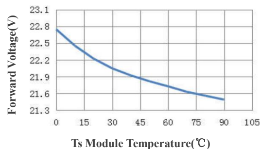
Temperature -VF Curve
